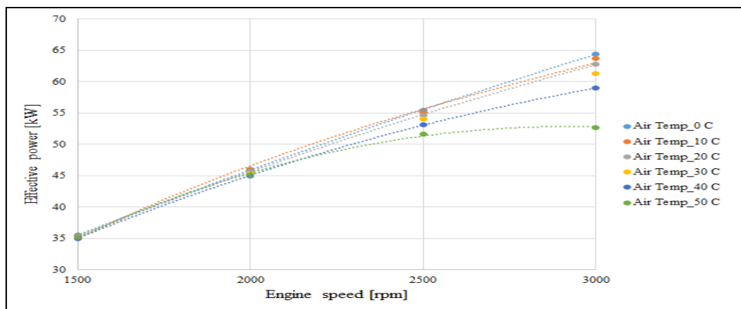
Fig.7. Effective power (KW) with engine speed (rpm) for multi inlet air temperature (°C) of GDI engine
