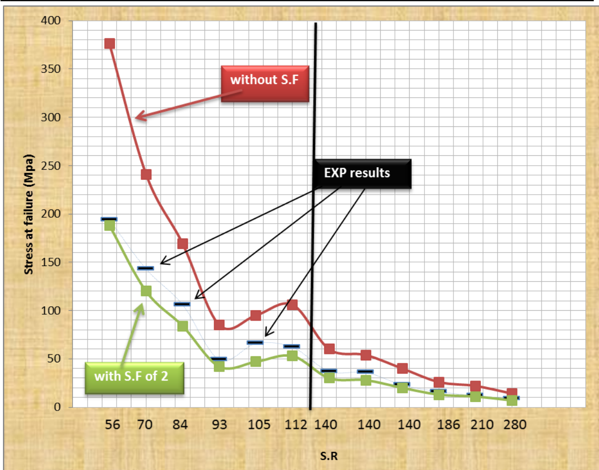
Figure (5) ANSYS curve with the experimental results for 304 stainless steel alloy
