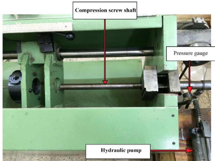
Figure (3) Compression machine section
