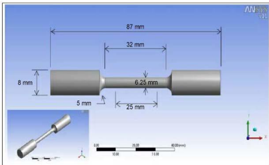
Figure (2) specimen dimensions of tensile test
