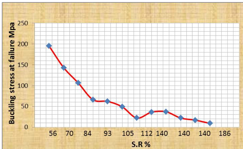
Figure (4) Dynamic compression buckling stress for (304 stainless steel alloy) for long columns
